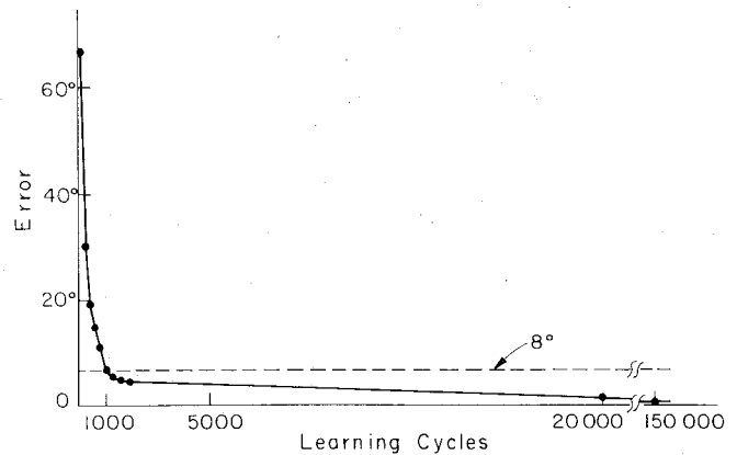
FIG. 9. Plot of the error of the output as a function of the number of training cycles. The distance between the receptive field centers of the retinal input units is 8^\circ ; an error of this magnitude is achieved after about 1000 repetitions.
