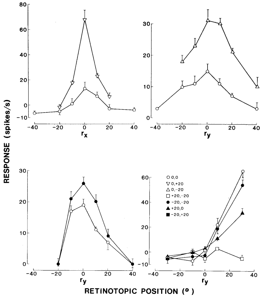
FIG. 4. Mean response rates for different eye positions plotted in retinal coordinates along horizontal ( r_x ) or vertical ( r_y ) axes passing through the centers of the receptive fields of four neurons; each graph shows data for one neuron. Each point represents the mean response ( \pm standard error) for eight repetitions of the stimulus presented at the same retinal location. A randomized block design was used to present stimuli to different retinal locations in the receptive field of each cell. The reported response at each retinal location is equal to the activity during the presentation of the stimulus minus the background activity determined before the stimulus presentation. From Andersen et al. (1985), reproduced from Science (Washington, DC), 230: 456-458, © AAAS.
